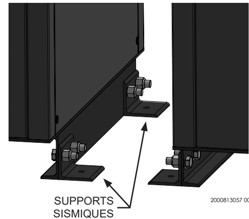
Figure 1-2 Supports sismiques
